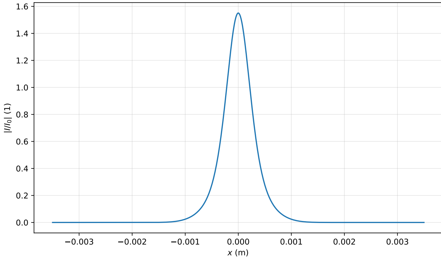
Intensity profile I(x, y = 0, z = 1.035m)/I_0 , P_{in}=1.0P_{cr} , artificial time
